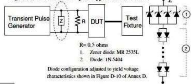
Figure 16-6: CI 220 Test setup for Application of Pulse G2
