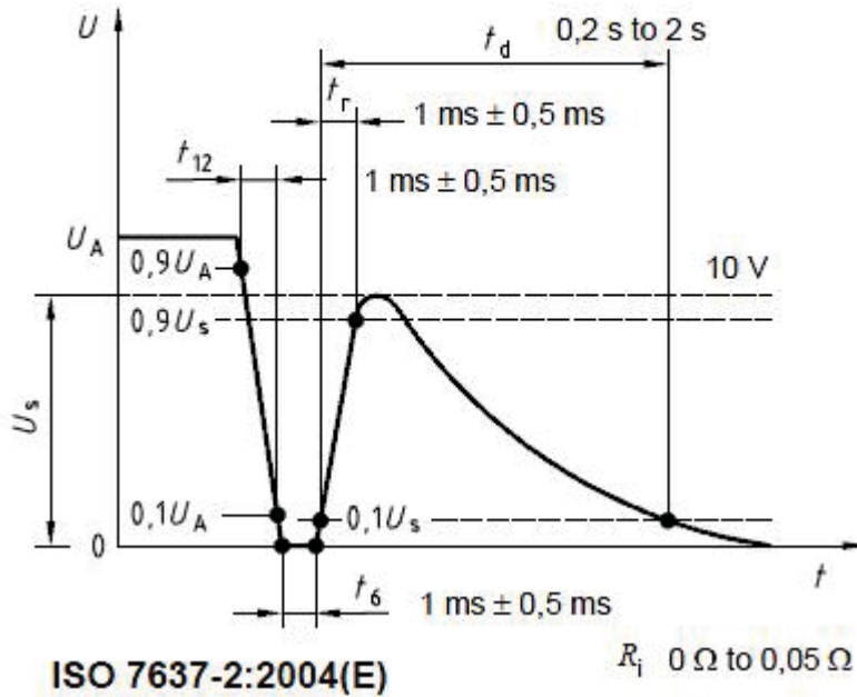
Figure 7 — Test pulse 2b 12 V system
